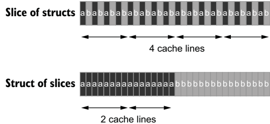
Figure 12.4 A struct of slices is more compact and therefore requires fewer cache lines to iterate over.
